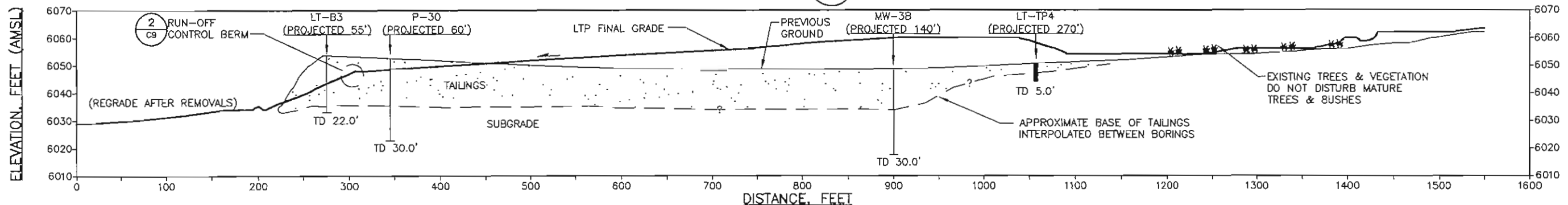
SECTION A C4
